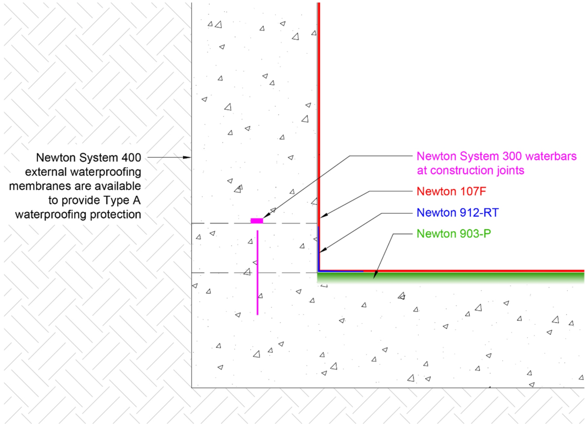
Figure 1 - Typical concrete joint detail
