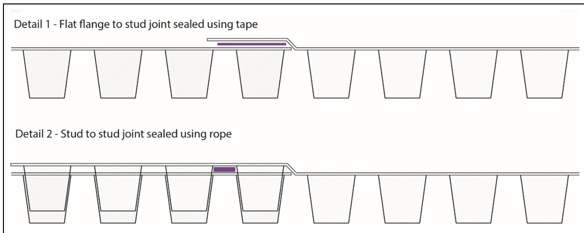
Figure 3 CDM Tape and CDM Rope sealing
